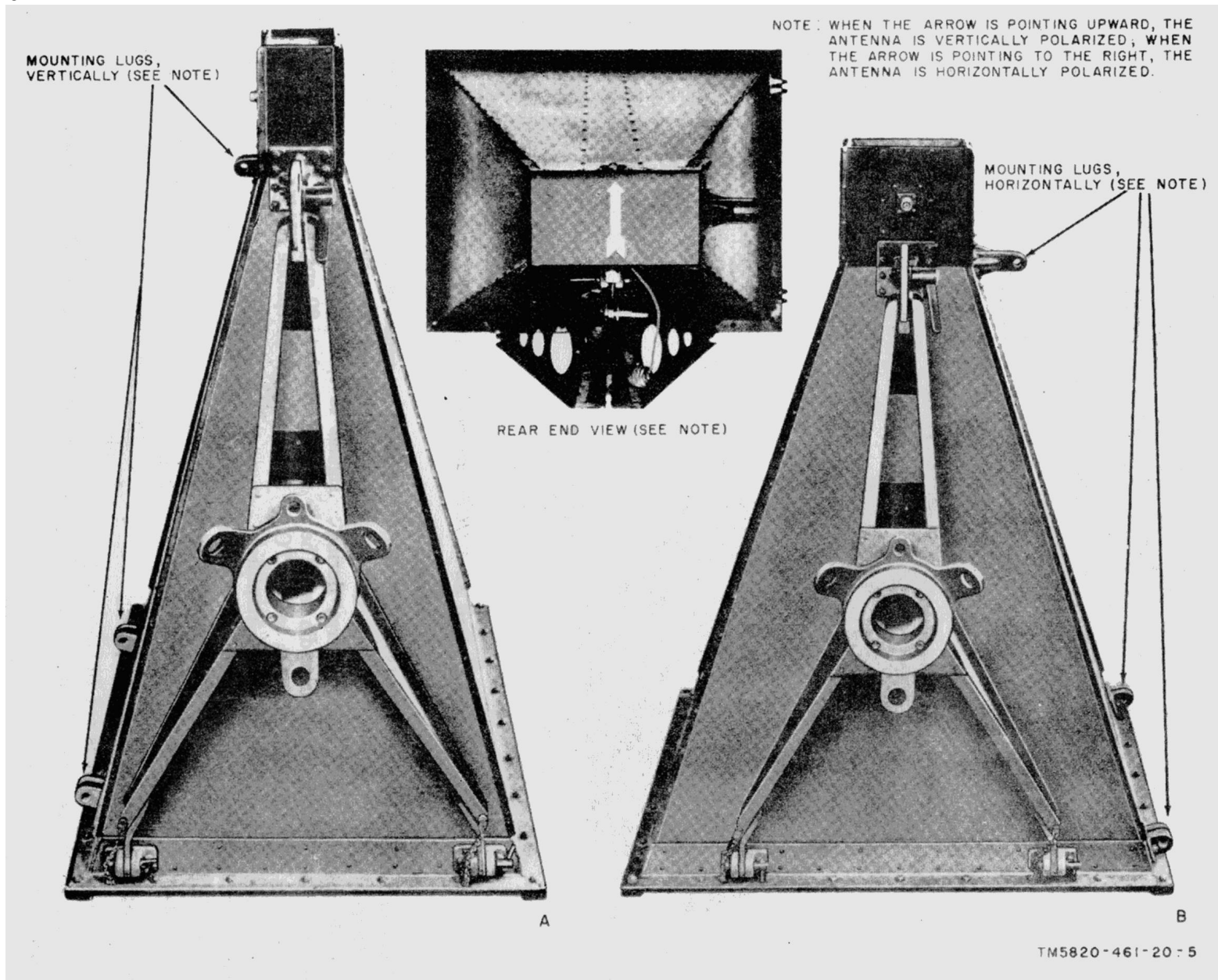
Figure 1-7. Antenna AT-903/G
